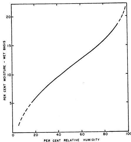
Figure 1. Equilibrium moisture content of wheat.
